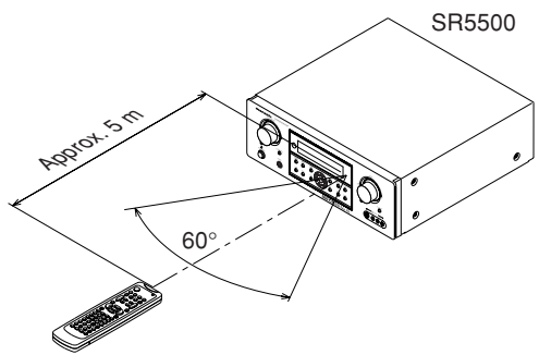
Remote control unit (RC5500SR)
